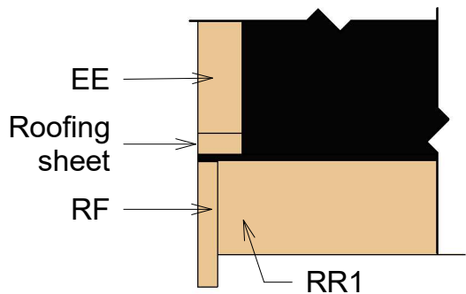
3 Roof Reinforcement
